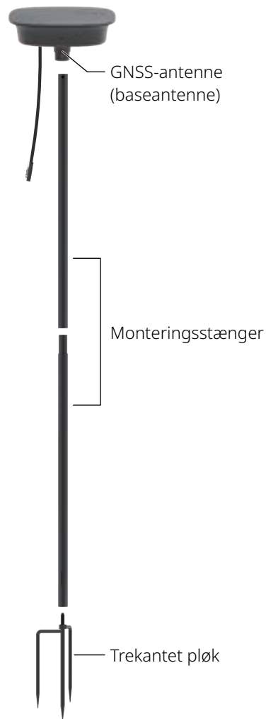
RTK-referencestation
